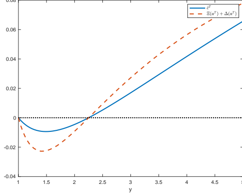
Figure 2: The blue solid line corresponds to \hat{c}^T whereas the orange dashed line represents the sum of the two externalities \Delta(a^T) + \Xi(a^T) . The two curves switch signs for the same value of y . The parameter values used for this simulation are \lambda = \beta = \tau_e = \tau_\eta = \tau_\theta = 1 , \tau_u = 30 , and 1 \leq y \leq 5 .
